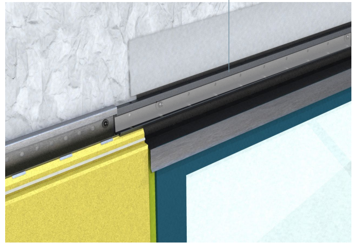
Starter Track over Z-flashing
