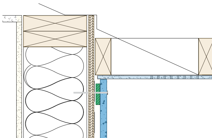
Soffit termination detail
