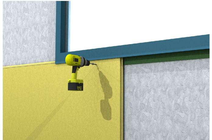
Face fasten the top edge of panels at sills.
